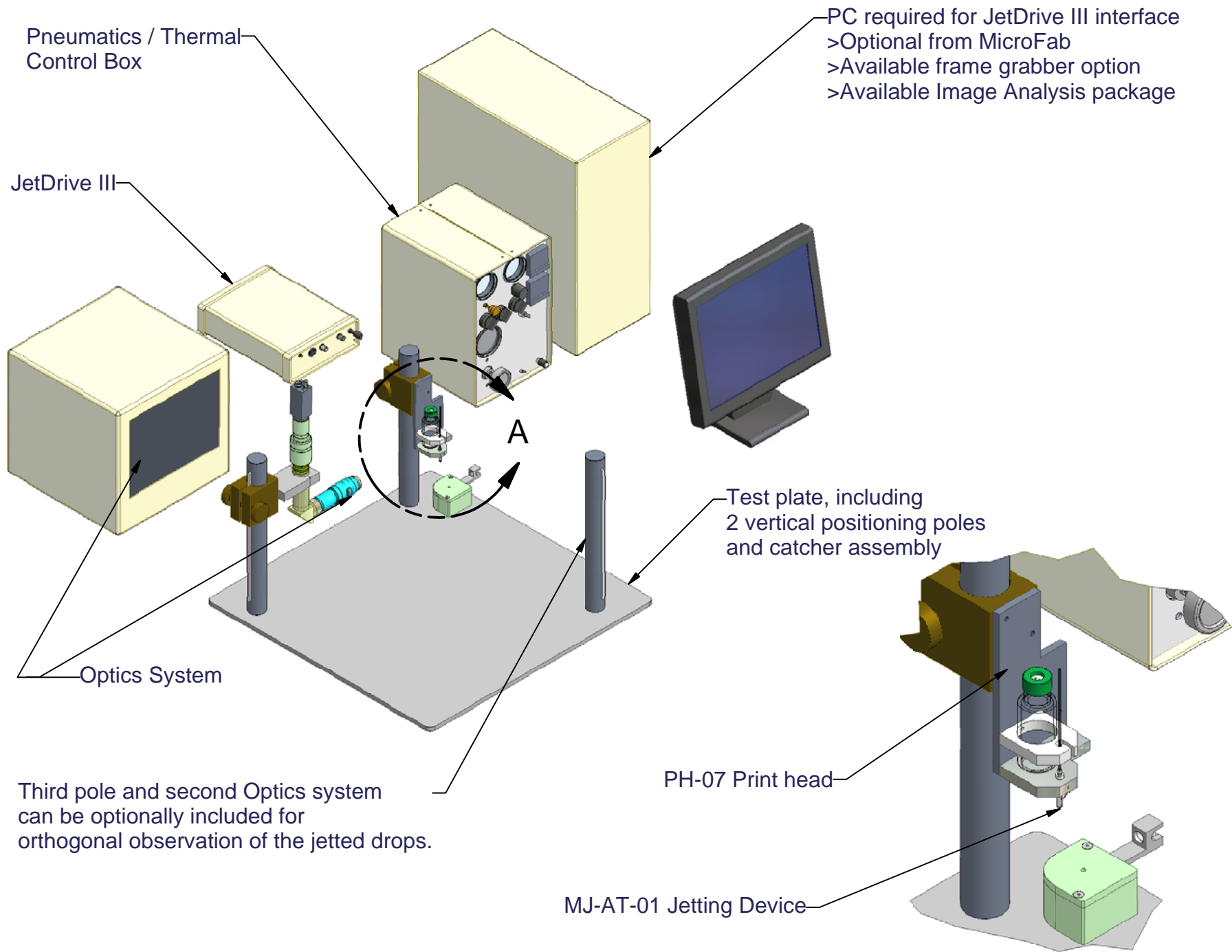
DETAIL A
